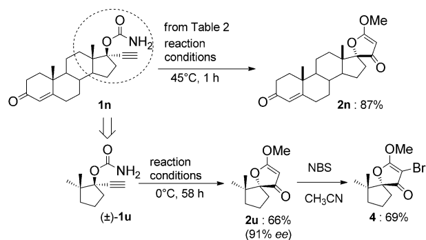
Scheme 4. First asymmetric reaction of racemic substrate ( \pm )- 1u in the presence of ( R,R )- L1 . Reaction conditions: ( R,R )- L1 (7.5 mol %), \text{Pd}(\text{tfa})_2 (5 mol %), p -benzoquinone (1.5 equiv), CO, MeOH.
